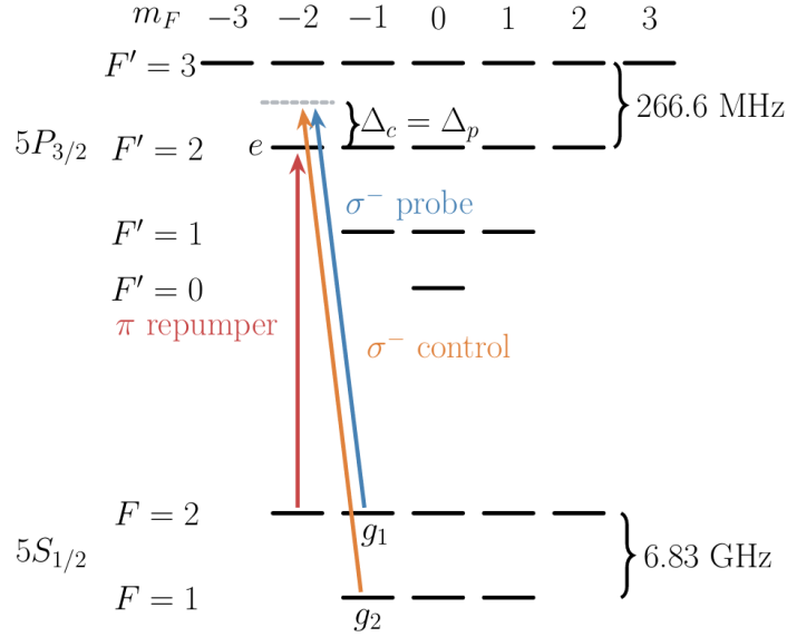
Figure 1.20: Level scheme of the ^{87}\text{Rb} D_2 transition implemented in the multilevel numerical model. The EIT \Lambda system is formed by the ground states |g_1\rangle = |F = 2, m_F = -1\rangle and |g_2\rangle = |F = 1, m_F = -1\rangle , both coupled to the excited state |e\rangle = |F' = 2, m_F = -2\rangle .
