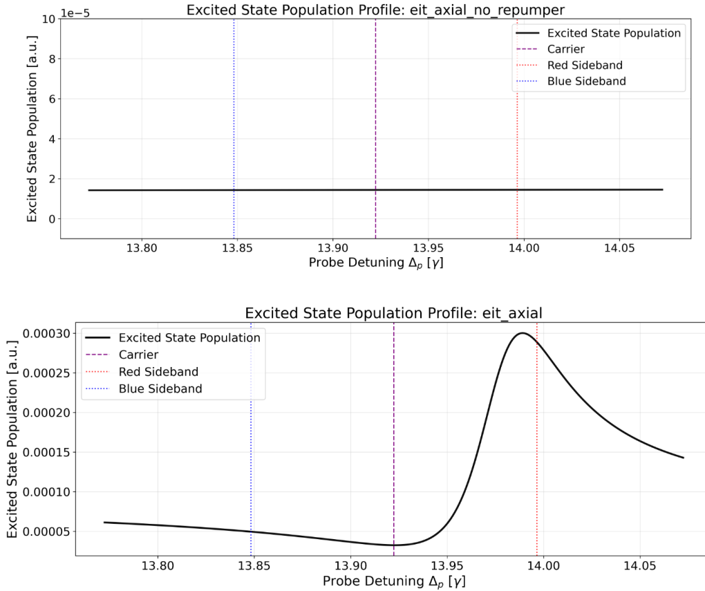
Figure 1.17: Comparison of the steady-state excited population in the 24-level system. Top: Without a repump field, optical pumping into dark states causes the spectroscopic signal to vanish. Bottom: With an active repump field, the Fano profile is restored, though broadened by off-resonant scattering.
