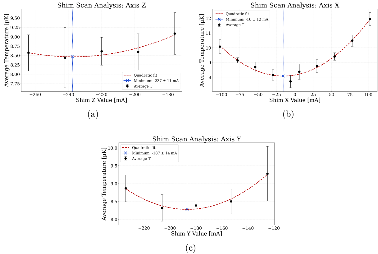
Figure 1.5: Optical molasses temperature as a function of the compensation currents. (a) Shim-Z scan: the minimum is located at I_z = -237 \pm 11 mA. (b) Shim-X scan: the parabolic fit indicates a minimum at I_x = -16 \pm 12 mA. (c) Shim-Y scan: the minimum is found at I_y = -187 \pm 14 mA.
