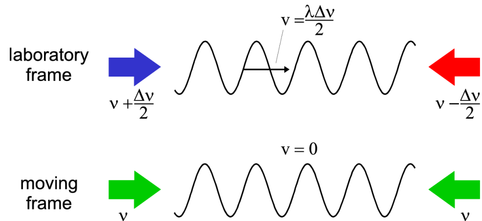
Figure 1.10: Kinematics of the optical conveyor belt: a mutual detuning \Delta\nu produces a moving standing wave. In the moving reference frame both beams are doppler shifted by the same amount [7].
