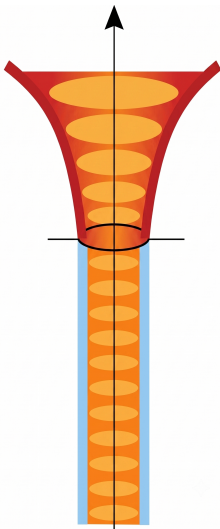
Figure 1.9: The strongly anisotropic, disc-shaped potential wells of the one-dimensional optical lattice.
