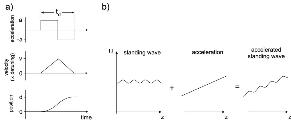
Figure 1.11: In the frame co-moving with the accelerated lattice, the periodic potential is superimposed with a linear gradient, resulting in a tilted washboard landscape [7].
