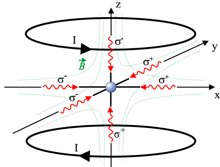
Figure 1.5: Schematic representation of the Magneto-Optical Trap (MOT) configuration, illustrating the counter-propagating laser beams with alternating \sigma^+/\sigma^- polarizations and the anti-Helmholtz coils used to generate the magnetic quadrupole field. From [7]
