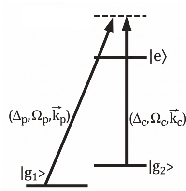
Figure 1.12: The three-level \Lambda system used for EIT cooling, consisting of two ground states ( |g_1\rangle, |g_2\rangle ) coupled to a common excited state ( |e\rangle ) by a probe and a coupling laser.
