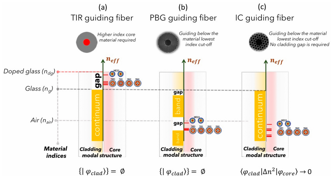
Figure 1.2: Schematic comparison of the internal reflection, PBG and IC guiding mechanisms. The effective index n_{\text{eff}} is plotted on the vertical axis, with the relevant index levels marked by horizontal dashed lines. The graphs display the cladding photonic bands versus n_{\text{eff}} , highlighting the core guidance regimes through continua (orange rectangles) and bandgaps (white rectangles). For TIR and PBG fibers, core modes are guided within the gaps. In contrast, IC fibers exhibit no bandgaps, and guidance occurs alongside the cladding mode continuum. Credits [6].
