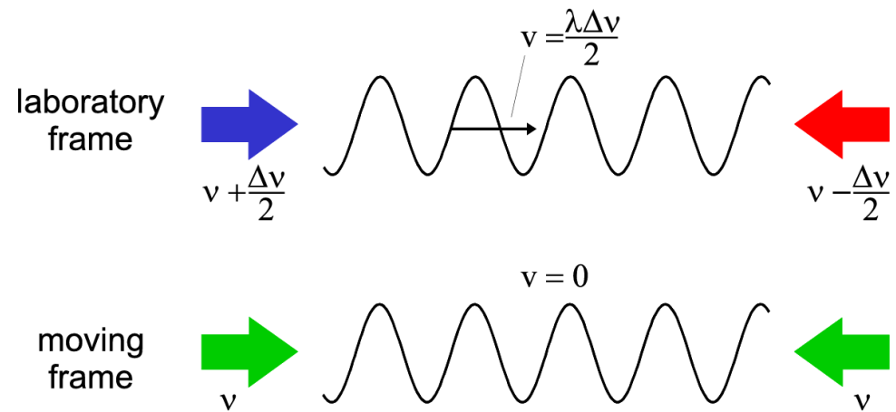
Figure 1.10: Kinematics of the optical conveyor belt: a mutual detuning \Delta\nu produces a moving standing wave. In the moving reference frame both beams are doppler shifted by the same amount [10].
