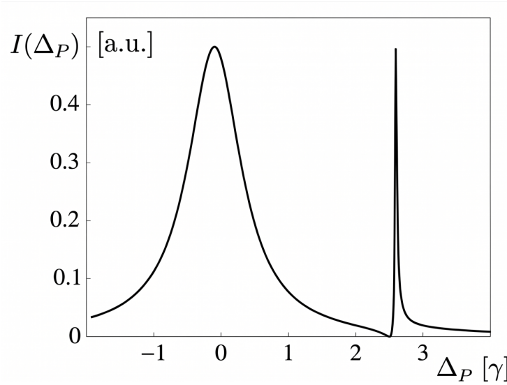
Figure 1.13: Absorption spectrum of the weak probe laser as a function of the two-photon detuning \delta_{2\text{ph}} = \Delta_p - \Delta_c , obtained by scanning \Delta_p while keeping the coupling detuning \Delta_c = \Delta fixed. The spectrum exhibits the characteristic asymmetric Fano lineshape of EIT: a zero-absorption point at \delta_{2\text{ph}} = 0 , a broad resonance of width \gamma_+ \approx \gamma associated with |\psi_+\rangle , and a narrow, AC-Stark-shifted resonance of width \gamma_- \ll \gamma associated with |\psi_-\rangle . Credits: [12]
