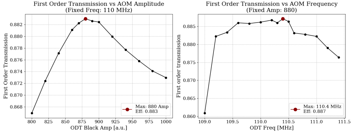
Figure 1.20: First-order transmission profile of the black-fiber branch AOM. The left panel shows the transmission as a function of the DDS amplitude (at a fixed frequency of 110 MHz, peaking at an amplitude setting of 880). The right panel shows the transmission as a function of the RF frequency (at a fixed amplitude of 880, peaking around 110.4 MHz).
