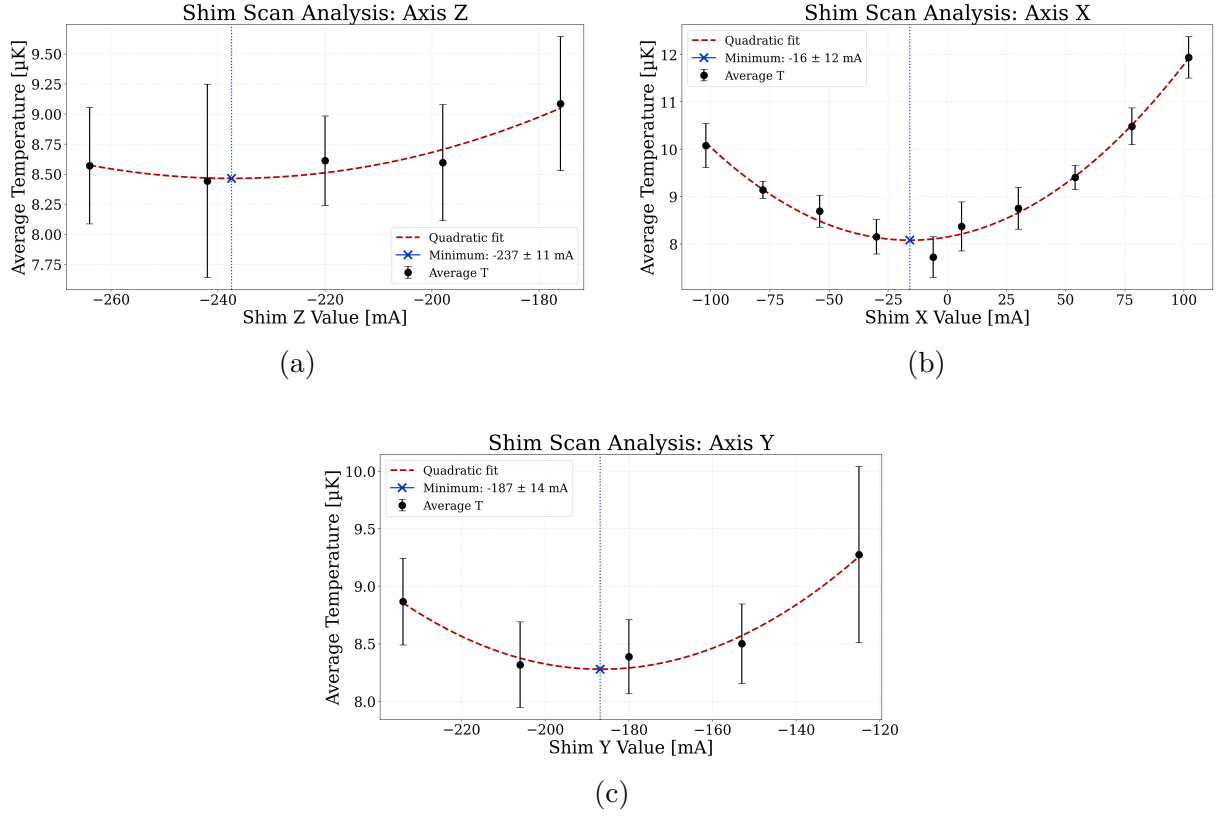
Figure 1.5: Optical molasses temperature as a function of the compensation currents. (a) Shim-Z scan: the minimum is located at I_z \approx -237.5 mA. (b) Shim-X scan: the parabolic fit indicates a minimum at I_x \approx -15.9 mA. (c) Shim-Y scan: the minimum is found at I_y \approx -186.9 mA.
