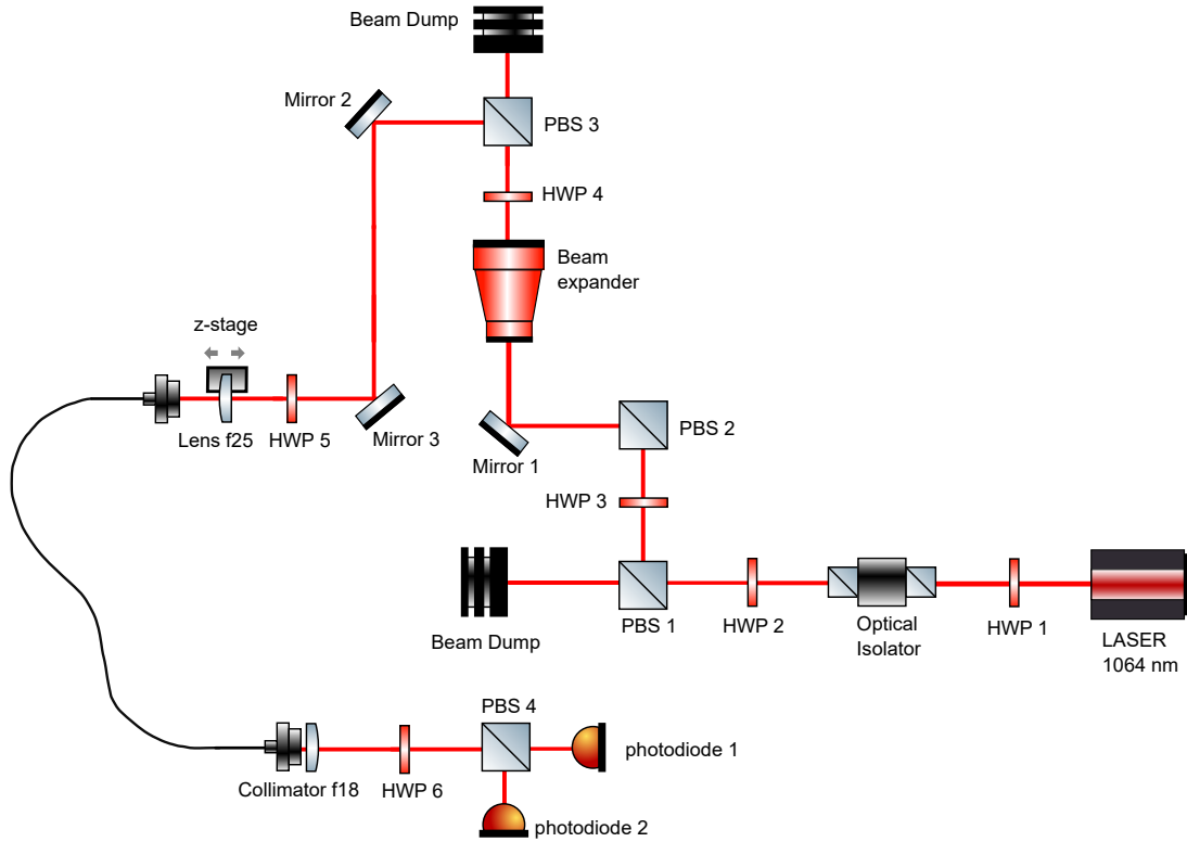
Figure 1.13: Setup of the black-fiber injection test bench, used to validate the mode-matching procedure and calibrate the axial position of the f = 25 mm lens. At the fiber output the polarization stability was characterized with the setup of Section 1.5.
