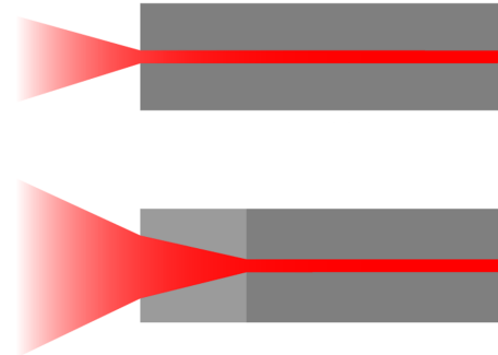
Figure 1.12: Geometry of the endcap spliced onto the black-fiber input. Image courtesy of Thorlabs, Inc.
