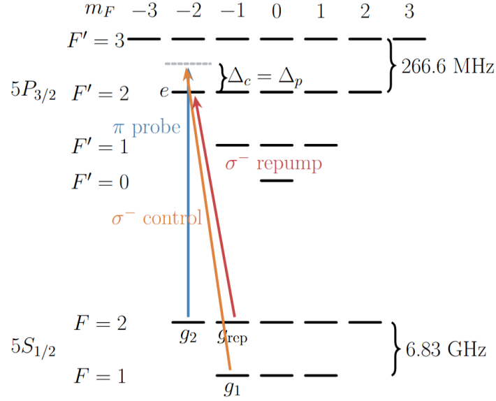
Figure 1.20: Level scheme of the ^{87}\text{Rb} D_2 transition implemented in the multilevel numerical model. The EIT \Lambda system is formed by the ground states |g_1\rangle = |F=1, m_F=-1\rangle and |g_2\rangle = |F=2, m_F=-2\rangle , both coupled to the excited state |e\rangle = |F'=2, m_F=-2\rangle .
