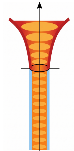
Figure 1.9: The strongly anisotropic, disc-shaped potential wells of the one-dimensional optical lattice.
