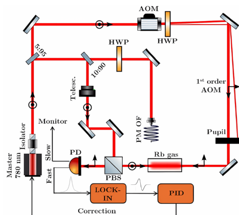
Figure 2.3: Master laser locking setup scheme.
