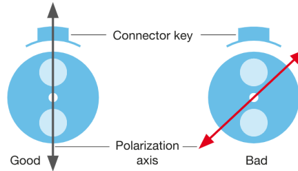
Figure 2.15: Orientation of the incident polarization relative to the slow and fast axes of the polarization-maintaining fiber.
