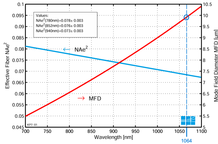
Figure 2.11: Manufacturer specification of the mode-field diameter of the black fiber. Add the operating wavelength and identify the value used in the mode-matching calculation.
