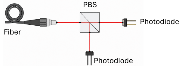
Figure 2.16: Setup used to characterize the polarization stability of the black fiber. The two orthogonal polarization components separated by the PBS are detected simultaneously and acquired on two independent channels.
