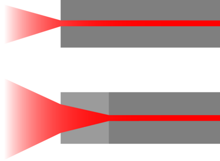
Figure 2.12: Geometry of the endcap spliced onto the black-fiber tip. Add the endcap length, connector orientation, and propagation direction.
