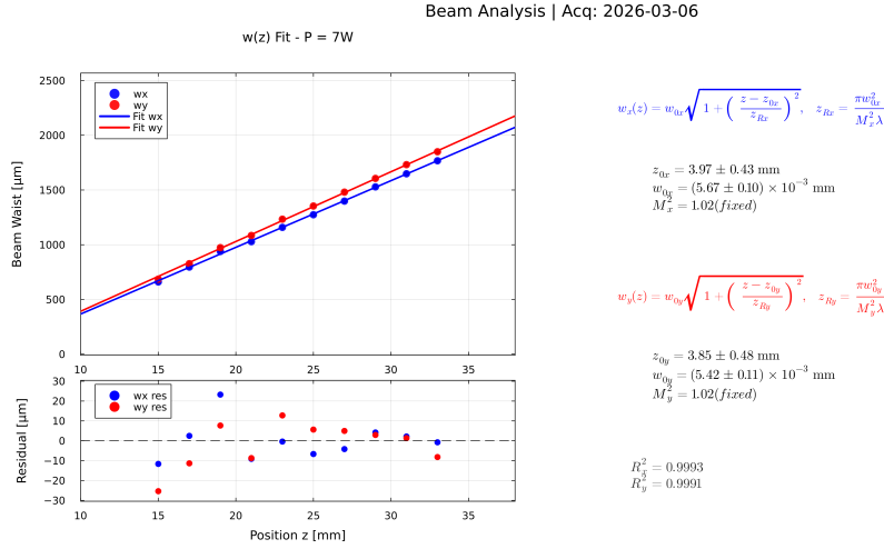
Figure 2.9: Beam-radius measurements after the black fiber and fit to the Gaussian-beam propagation law. Complete the caption with the measurement direction, fitting parameters, uncertainties, and optical configuration.
