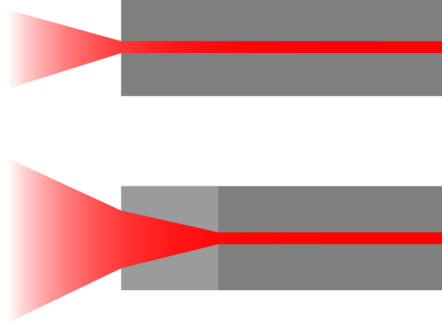
Figure 2.11: Geometry of the endcap spliced onto the black-fiber tip. Add the endcap length, connector orientation, and propagation direction.
