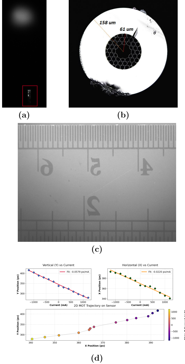
Figure 2.6: Summary of the three spatial-calibration methods used for the imaging system. (a) Side-view photograph of the hollow-core photonic crystal fiber (HCPCF) used as the known-length reference for Method 1; the apparent diameter is fitted to extract the effective pixel size. (b) Cross-section of the same fiber, with its 316\,\mu\text{m} physical diameter annotated, used together with (a) in Method 1. (c) Photograph of the ruler whose reflected image is brought into focus at the cloud plane, used in Method 2 (optical target calibration via reflection). (d) MOT position as a function of the bias current applied to the y-axis shim coils, used in Method 3 (magnetic field displacement); the linear fit gives a slope of \sim 58\,\text{px/A} , from which the effective pixel size C \approx 43\,\mu\text{m/px} is obtained. The two side-view images (a) and (c) are taken from the actual recorded frames, while (b) is a fiber cross-section schematic.
