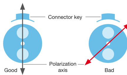
Figure 2.13: Orientation of the incident polarization relative to the slow and fast axes of the polarization-maintaining fiber.
