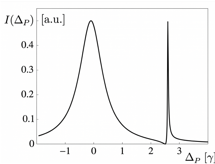
Figure 1.13: Absorption spectrum obtained by scanning \Delta_p while keeping the coupling detuning \Delta_c = \Delta fixed. The spectrum exhibits the characteristic asymmetric Fano lineshape of EIT: a zero-absorption point at \delta_{2\text{ph}} = 0 , a broad resonance of width \gamma_- \approx \gamma associated with |\psi_- \rangle , and a narrow, AC-Stark-shifted resonance of width \gamma_+ \ll \gamma associated with |\psi_+ \rangle . Credits: [15].
