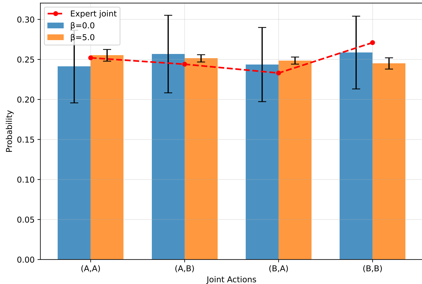
Final Joint Action Distribution
