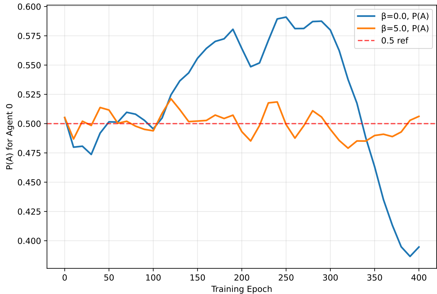
Policy Evolution During Training
