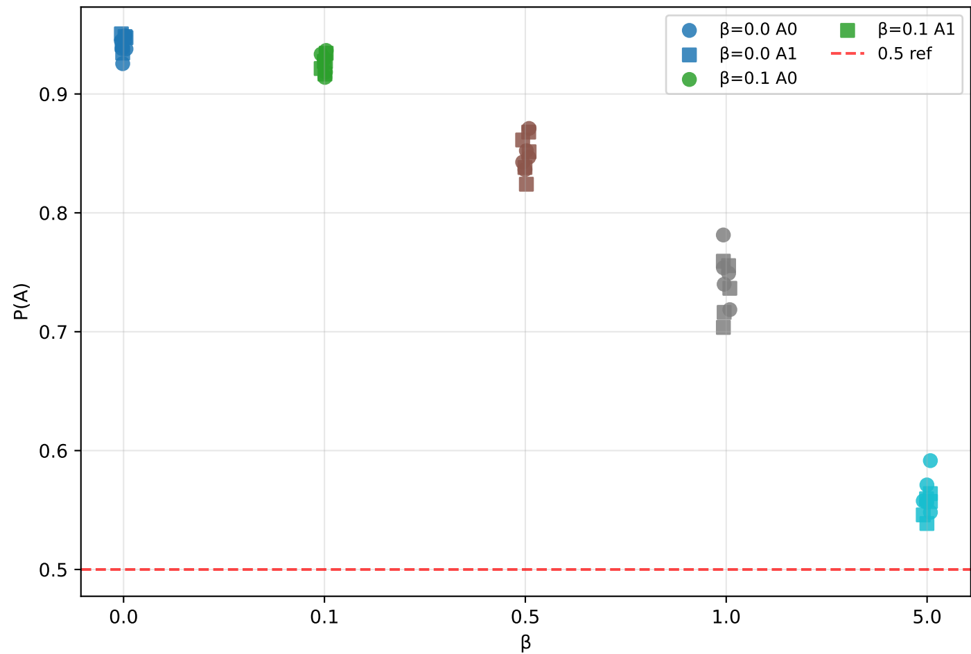
Final Policy Probabilities Across Seeds
