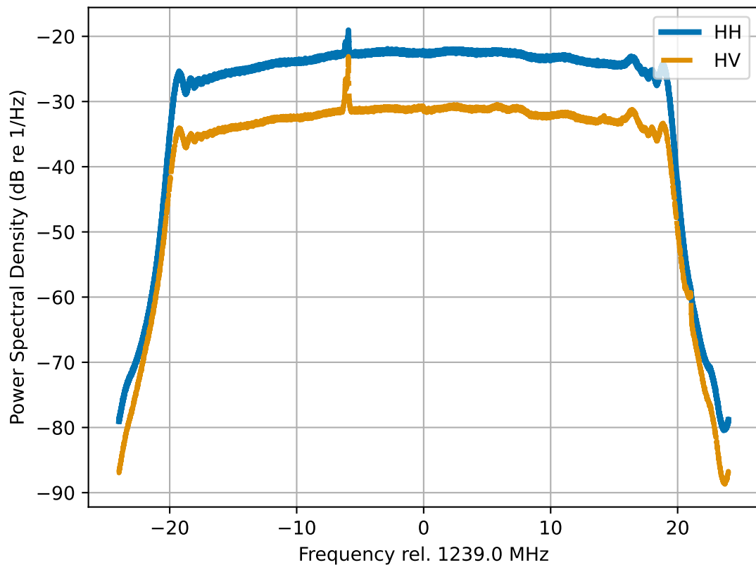
Range Power Spectra for Frequency A
