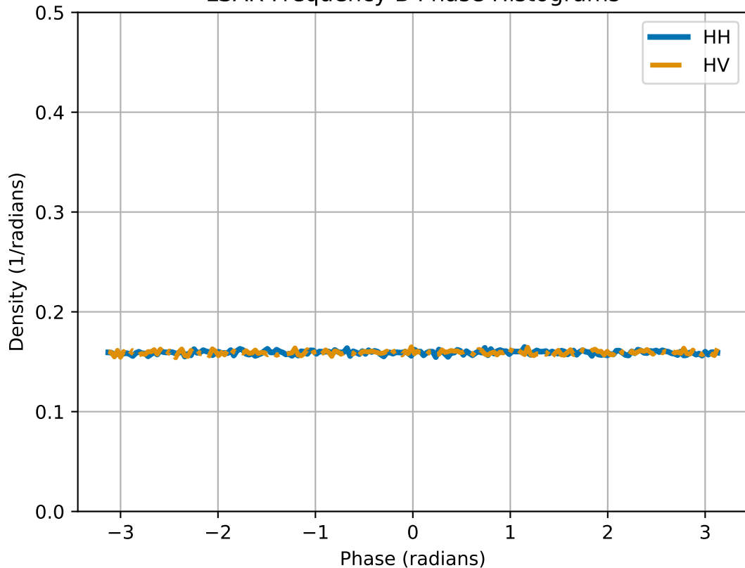
LSAR Frequency B Phase Histograms
