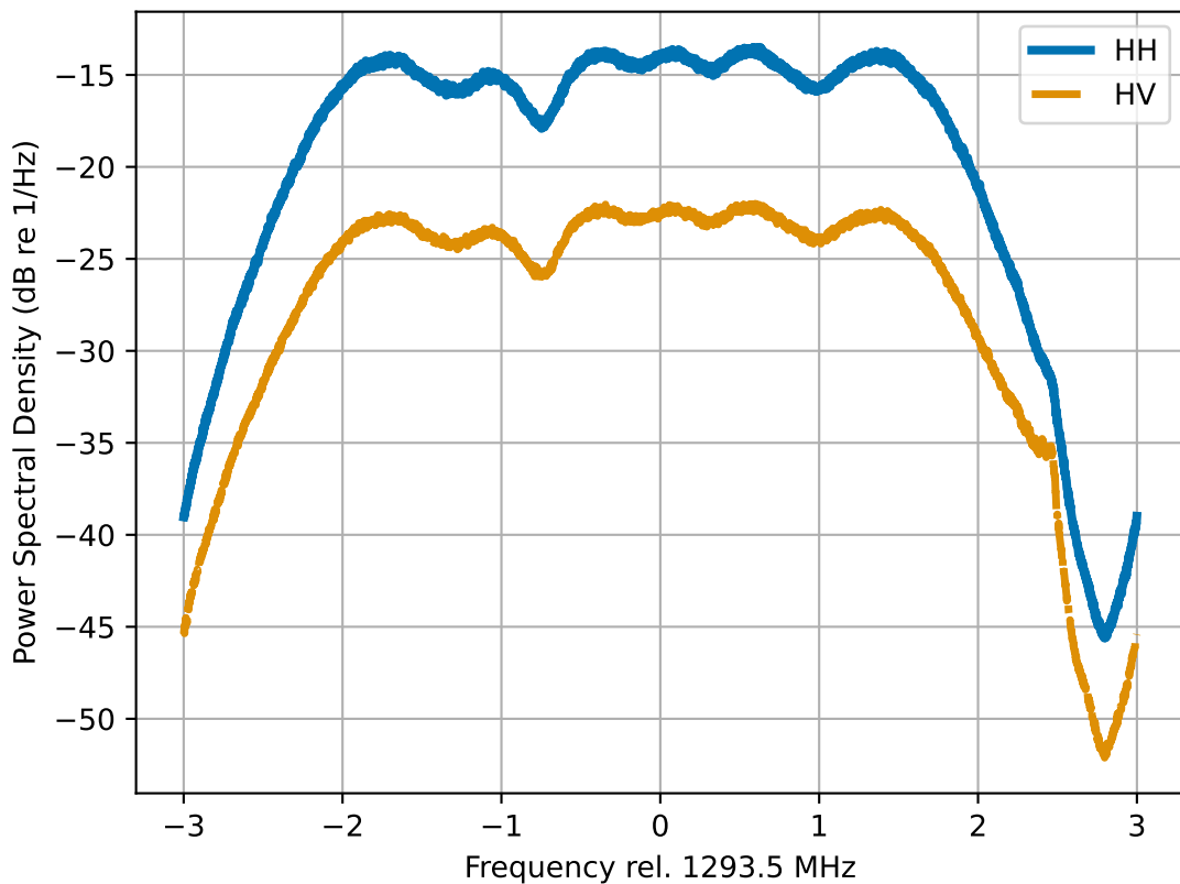
Range Power Spectra for Frequency B
