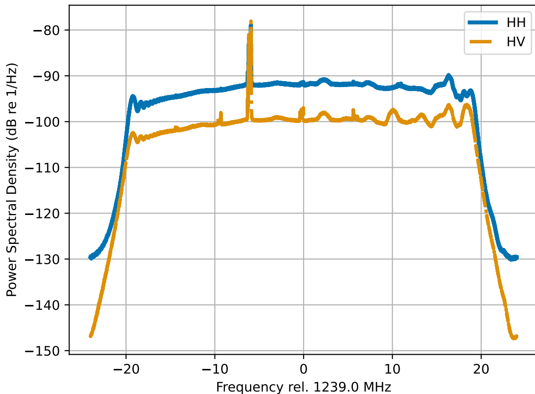
Range Power Spectra for Frequency A
