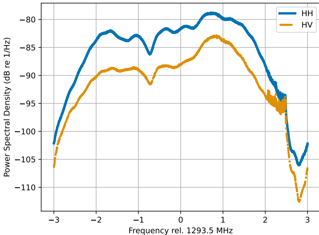
Range Power Spectra for Frequency B
