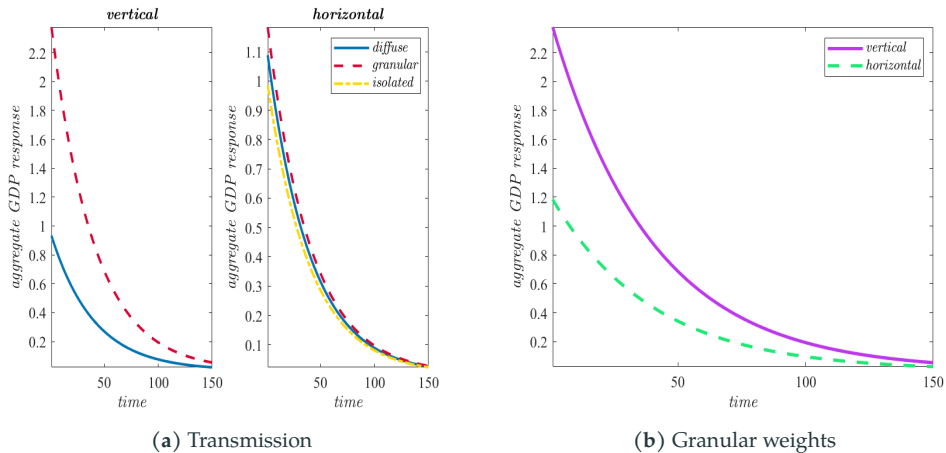
Figure 3: Aggregate fluctuations
