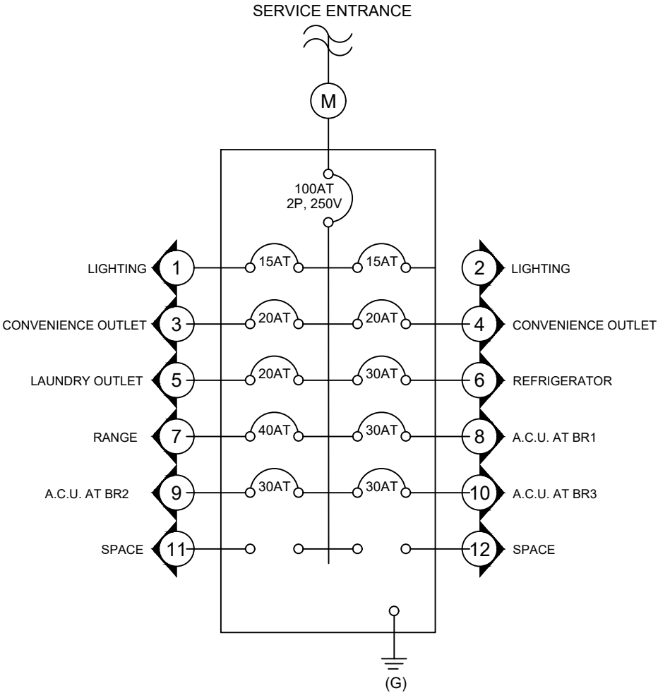
SINGLE LINE DIAGRAM
