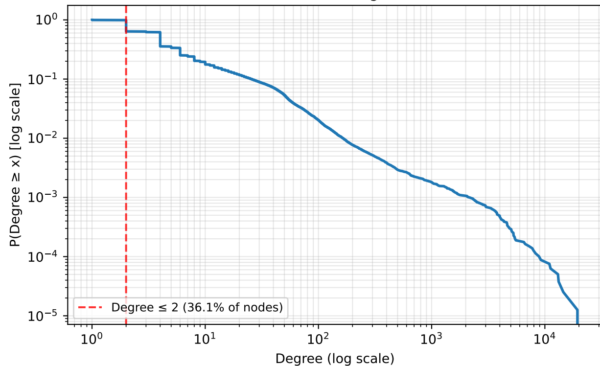
Degree Distribution (CCDF) Power-law long tail
