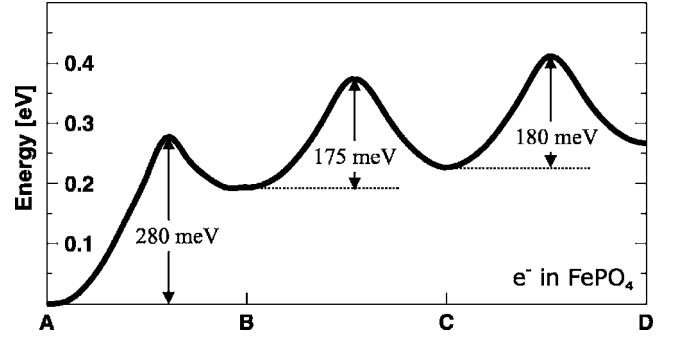
FIG. 4. Total energy along polaron migration path in \text{Li}(\text{FePO}_4)_{64} along four adjacent iron sites from \text{Fe}_A to \text{Fe}_D ( U = 4.3 eV). The distances between the \text{Li}^+ ion and the corresponding iron site are r_A = 3.18 Å, r_B = 5.50 Å, r_C = 9.18 Å, and r_D = 12.72 Å, respectively.
