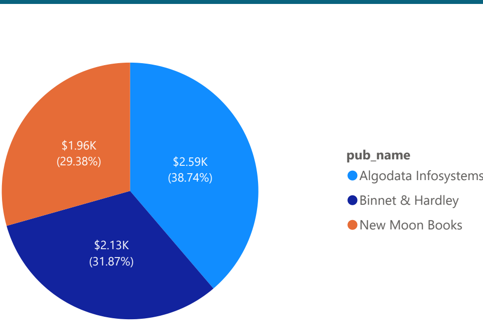
SaleAmountByPublisher
