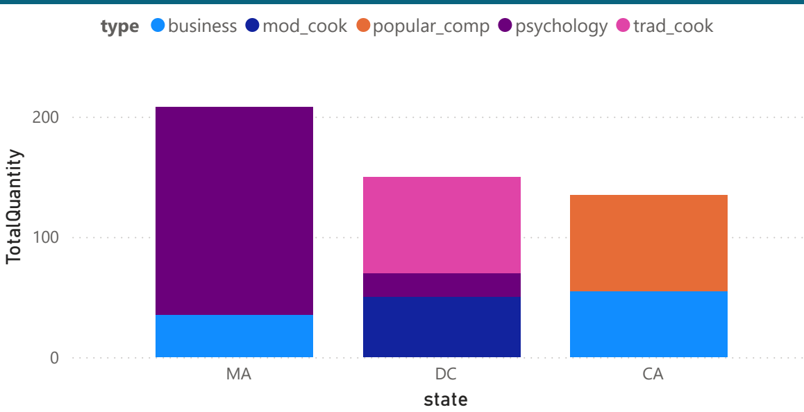
TitleQuantity
