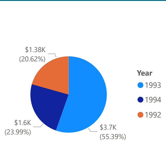
YearlySaleAmount
