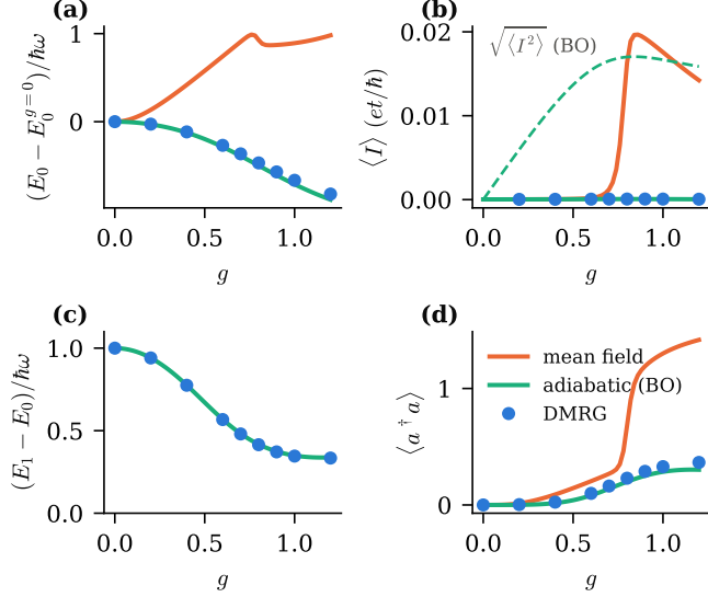
FIG. 3. Short ring with a Zeeman-polarized dot ( \hbar\omega = 0.02 , \varphi_{\text{cl}} = 10^{-3} ): mean field (MF, orange), adiabatic theory (3) (green), and DMRG (symbols). (a) Ground-state energy, (b) current (dashed: rms current of the BO ground state), (c) gap to the first excited state, (d) photon number.
