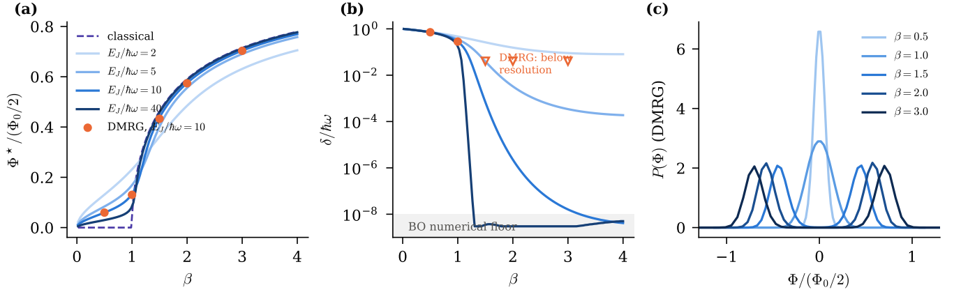
FIG. 5. Interaction-driven \pi loop ( U = 2t , no external flux). (a) Flux of the condensate \Phi^* (eigenvalue of the flux projected on the two lowest states) versus \beta for increasing E_J/\hbar\omega (lines: adiabatic theory with the DMRG E(\varphi) ; circles: full DMRG at E_J/\hbar\omega = 10 ; dashed: classical). (b) Tunnel splitting \delta between the two current-carrying states. (c) Flux distribution of the DMRG ground state (a cat state for \beta > 1 ).
