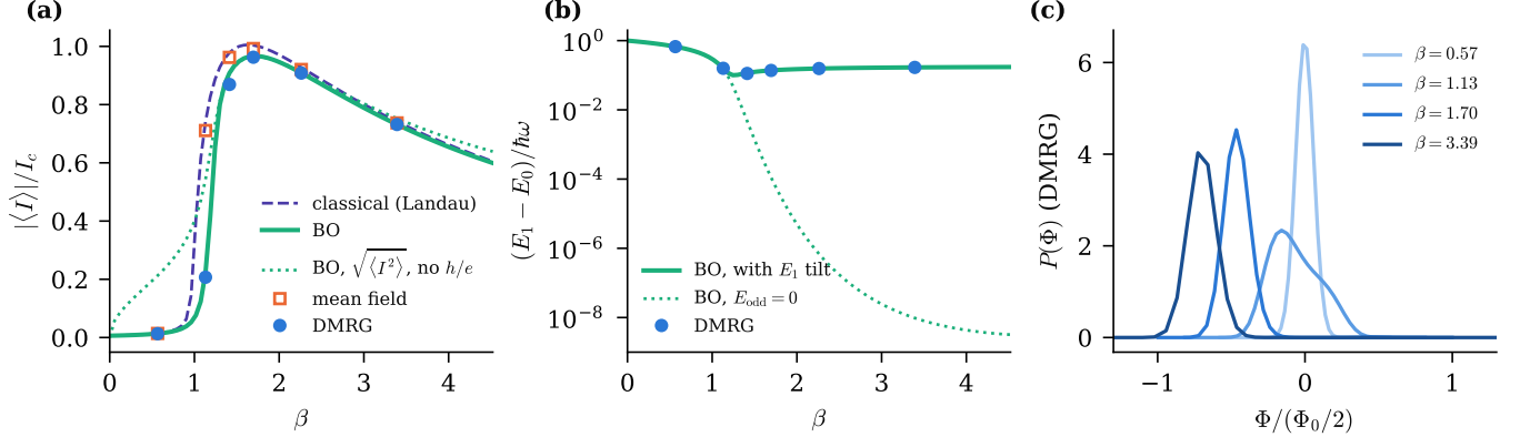
FIG. 4. Weak-link loop biased by \Phi_0/2 , E_J/\hbar\omega = 10 . (a) Persistent current versus \beta : DMRG (circles), MF (squares), adiabatic theory with (solid) and without (dotted) the odd harmonics, classical Landau theory (dashed). (b) Splitting of the two lowest levels. (c) Flux distribution of the DMRG ground state, obtained from the photon reduced density matrix.
