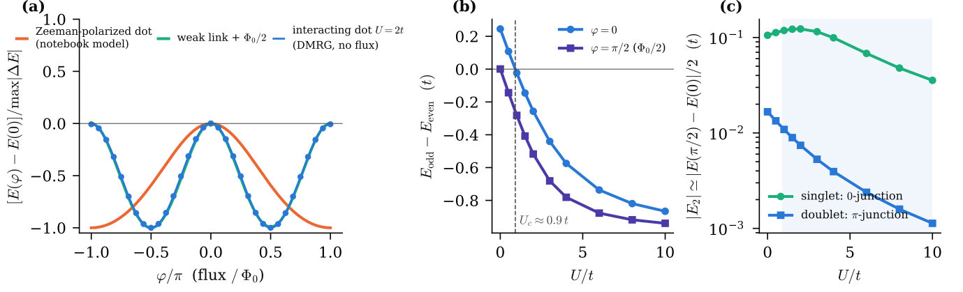
FIG. 2. (a) Normalized ground-state energy of the loop versus the electron phase \varphi (flux in units of h/2e ) for three junctions: Zeeman-polarized dot in a short ring (dominated by the single-electron harmonic \cos \varphi ), an ordinary weak link biased by \Phi_0/2 , and an interacting-dot ring at U = 2t without any bias (DMRG, symbols; line: cosine fit). (b) Parity competition E_{\text{odd}} - E_{\text{even}} of the interacting-dot ring at \varphi = 0 and \varphi = \pi/2 (DMRG, L = 14 , \Delta = t , t_J = 0.5t ). (c) Josephson energy |E_2| in the singlet (0) and doublet ( \pi ) sectors. Shading: doublet ground state.
