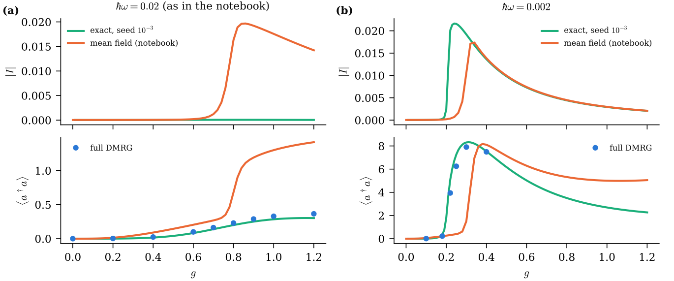
FIG. 3. Model of the original notebook (Zeeman-polarized dot, L = 11 , t = 2 , \Delta = 0.6 ): current (top) and photon number (bottom) versus g for (a) \hbar\omega = 0.02 and (b) \hbar\omega = 0.002 . Green: exact (adiabatic, seed 10^{-3} ); orange: mean field; circles: full DMRG.
