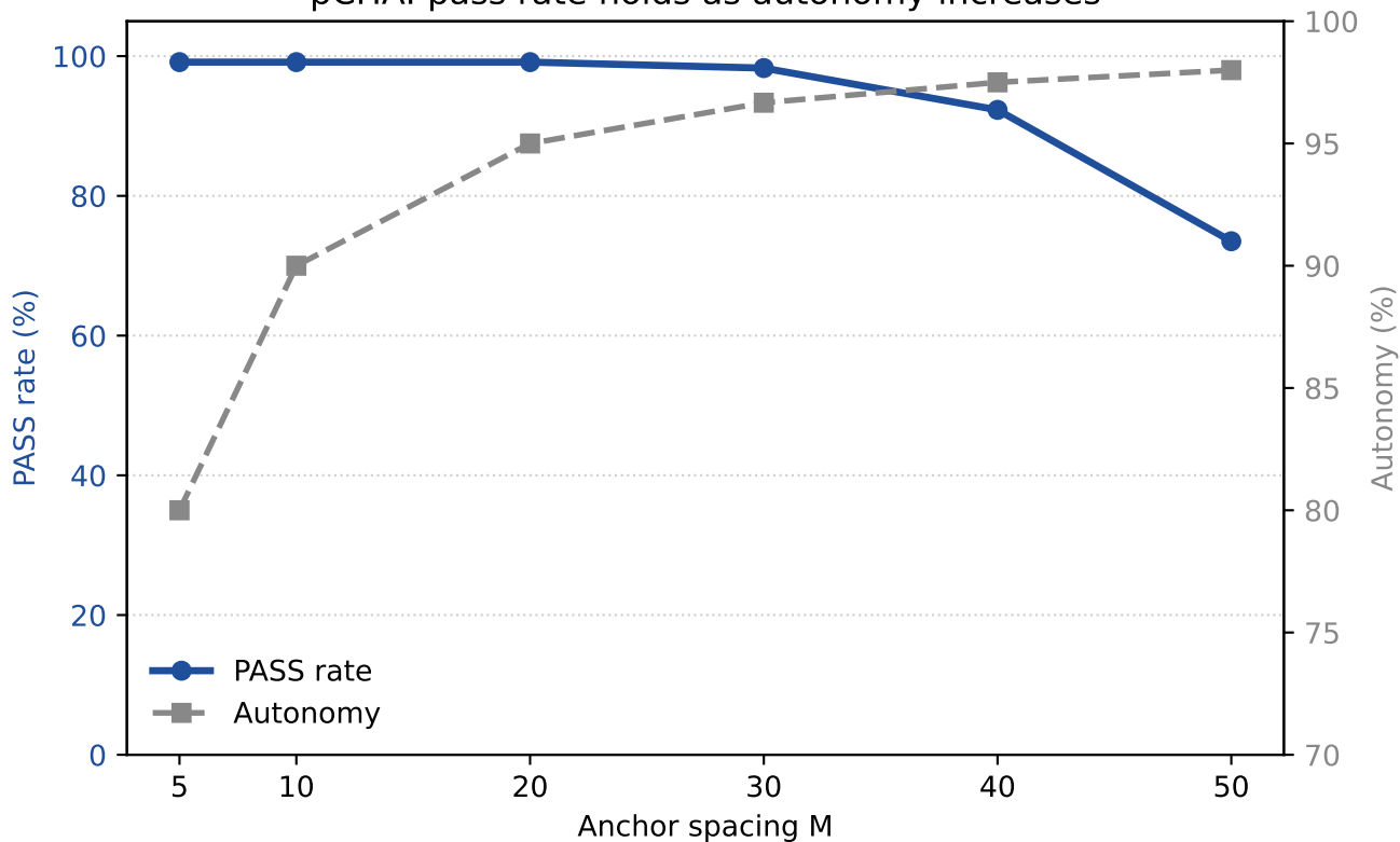
pCHA: pass rate holds as autonomy increases
