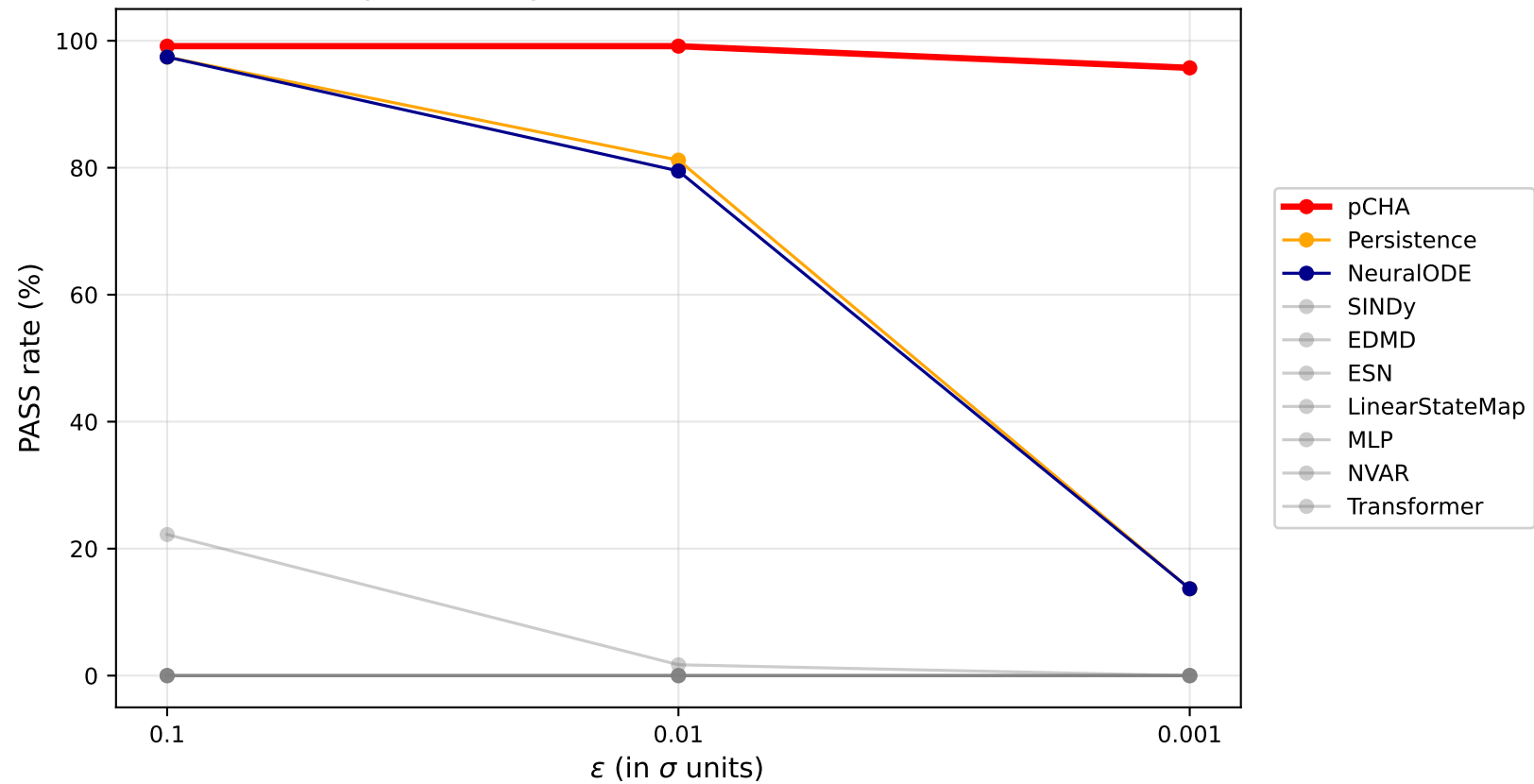
dysts (117 systems): PASS rate vs threshold
