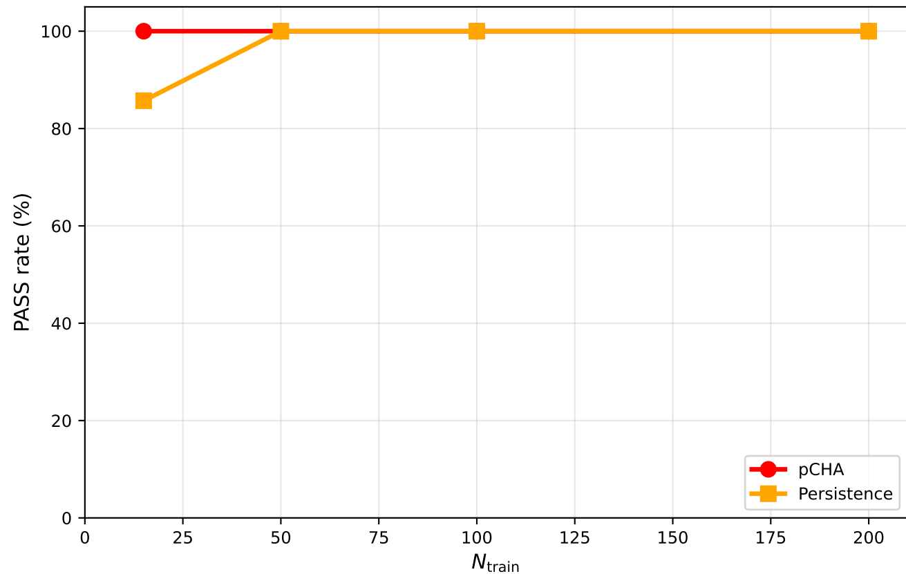
Real-world (7 datasets): PASS vs N_{\text{train}}
