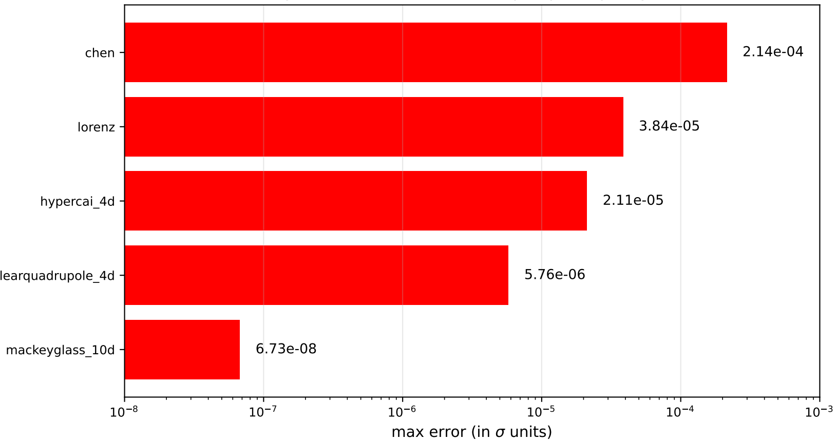
Long-horizon T=9900 (9.9M steps): pCHA per-system
