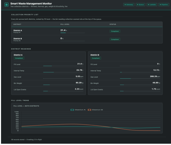
Fig. 2. The deployed Smart Waste Management Monitor dashboard, served from Amazon S3, showing the collection priority list, live readings for all five sensor types in both districts, the fill-level trend, and the four pipeline health indicators.
