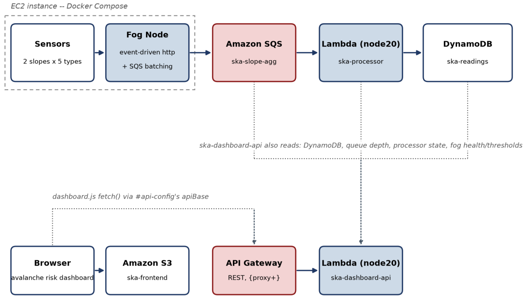
Fig. 1. Deployment topology. Sensors, fog node, SQS, ska-processor, and DynamoDB form the ingest path along the top; browser, S3, API Gateway, and ska-dashboard-api form the query path along the bottom. Only the EC2-hosted sensor and fog tier sits outside a managed AWS service.
