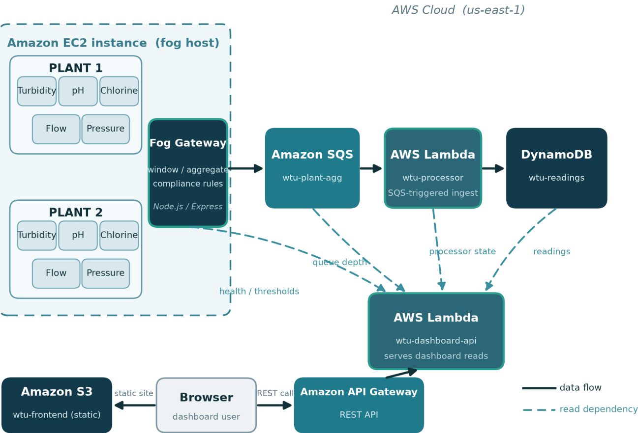
Fig. 1. Deployed fog-to-cloud topology. A single edge host at the plant runs the fog gateway and ten sensor containers. The solid path traces ingestion, from the instruments through the queue and the ingestion function into the table. The dashed paths are the four sources the dashboard function reads, the gateway, the queue, the ingestion function, and the table. Static assets reach the browser from object storage, and the browser calls the dashboard interface via the managed gateway.
