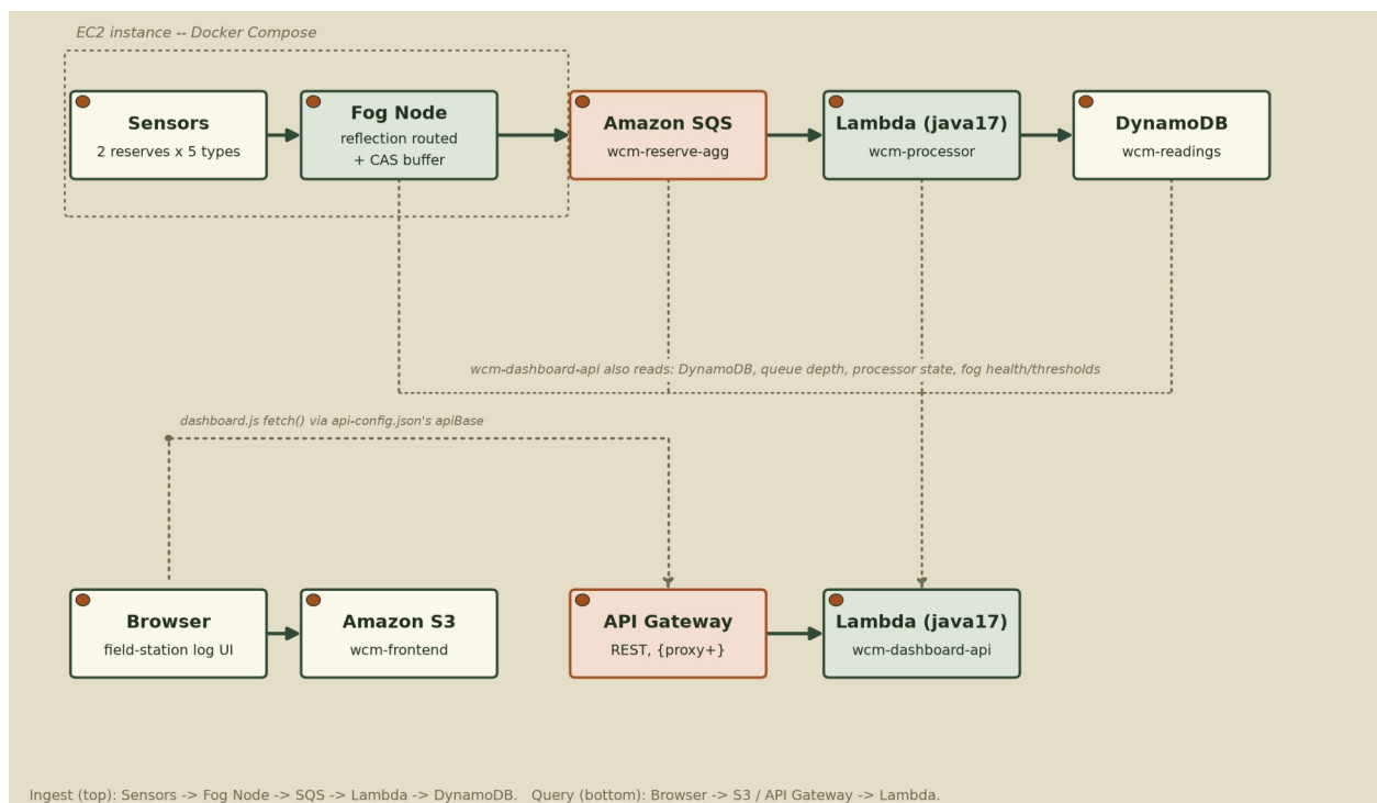
Fig. 1. Deployment topology: an ingest row (sensors through DynamoDB ) and a query row (browser through the dashboard API), with the EC2 -hosted sensor and fog tier the only piece not behind a managed AWS service.
