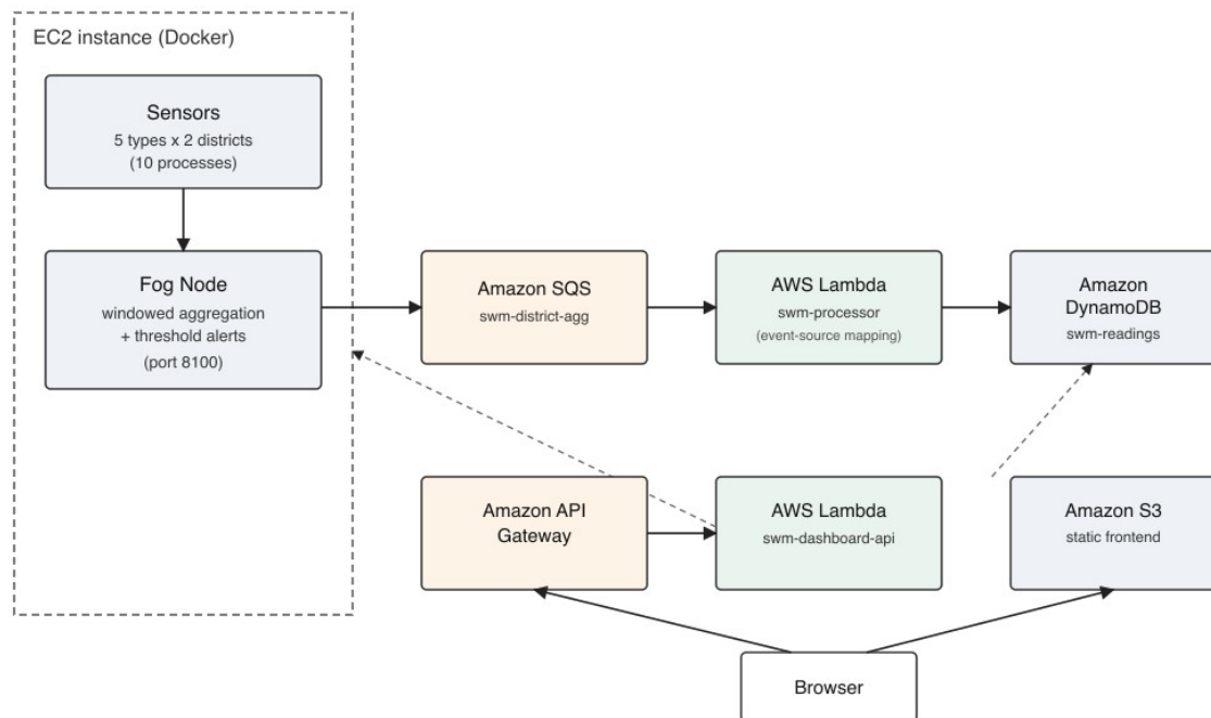
Fig. 1. Deployment topology: sensors and the fog node run on EC2; the backend (SQS, both Lambda functions, DynamoDB, API Gateway) is fully serverless; the frontend is served from S3.
