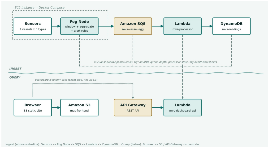
Fig. 1. Deployment topology: an ingest lane (sensors through DynamoDB) and a query lane (browser through the dashboard API) either side of a waterline; the backend is fully serverless except the EC2-hosted sensor and fog tier.
