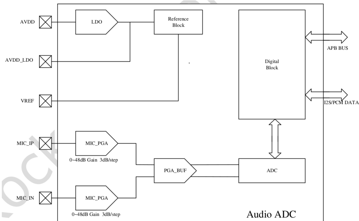
RV1126B/RV1126BP ACodec Block Diagram
