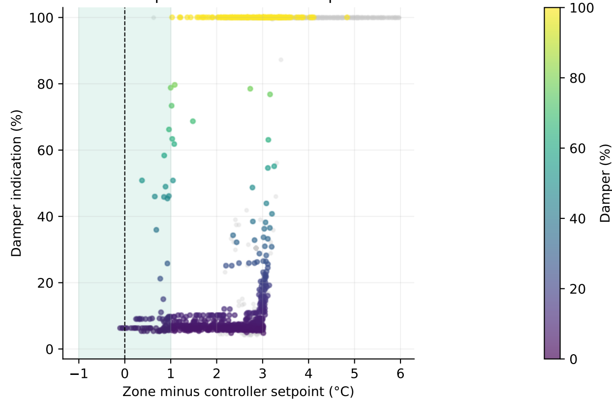
Temperature error vs damper
