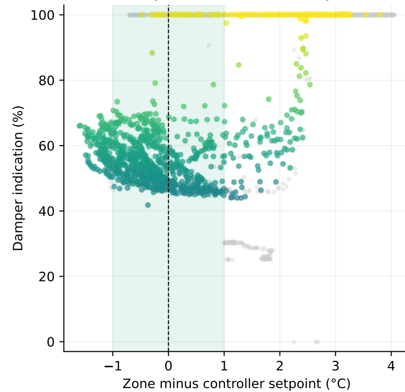
Temperature error vs damper
