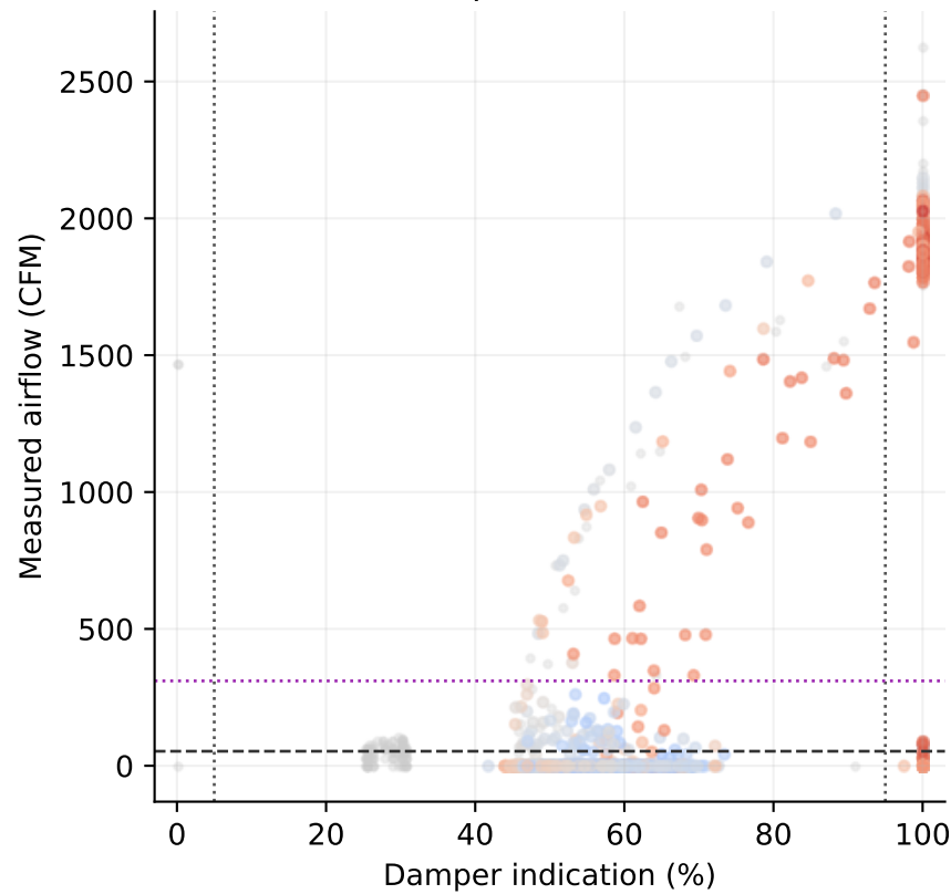
Damper vs airflow
