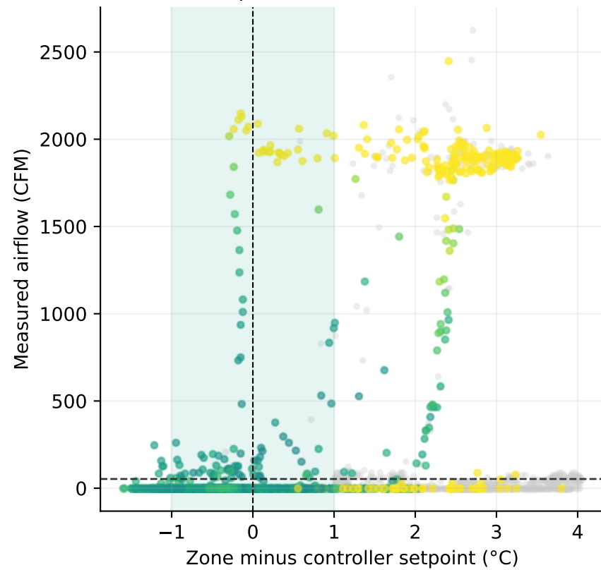
Temperature error vs airflow
