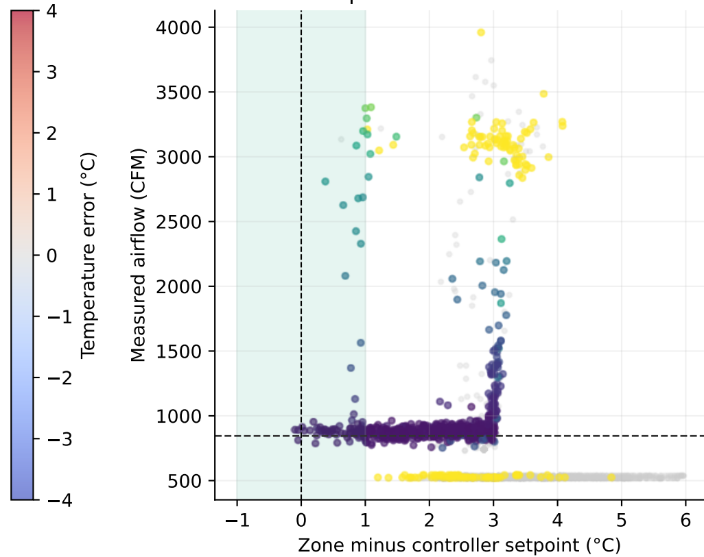
Temperature error vs airflow
