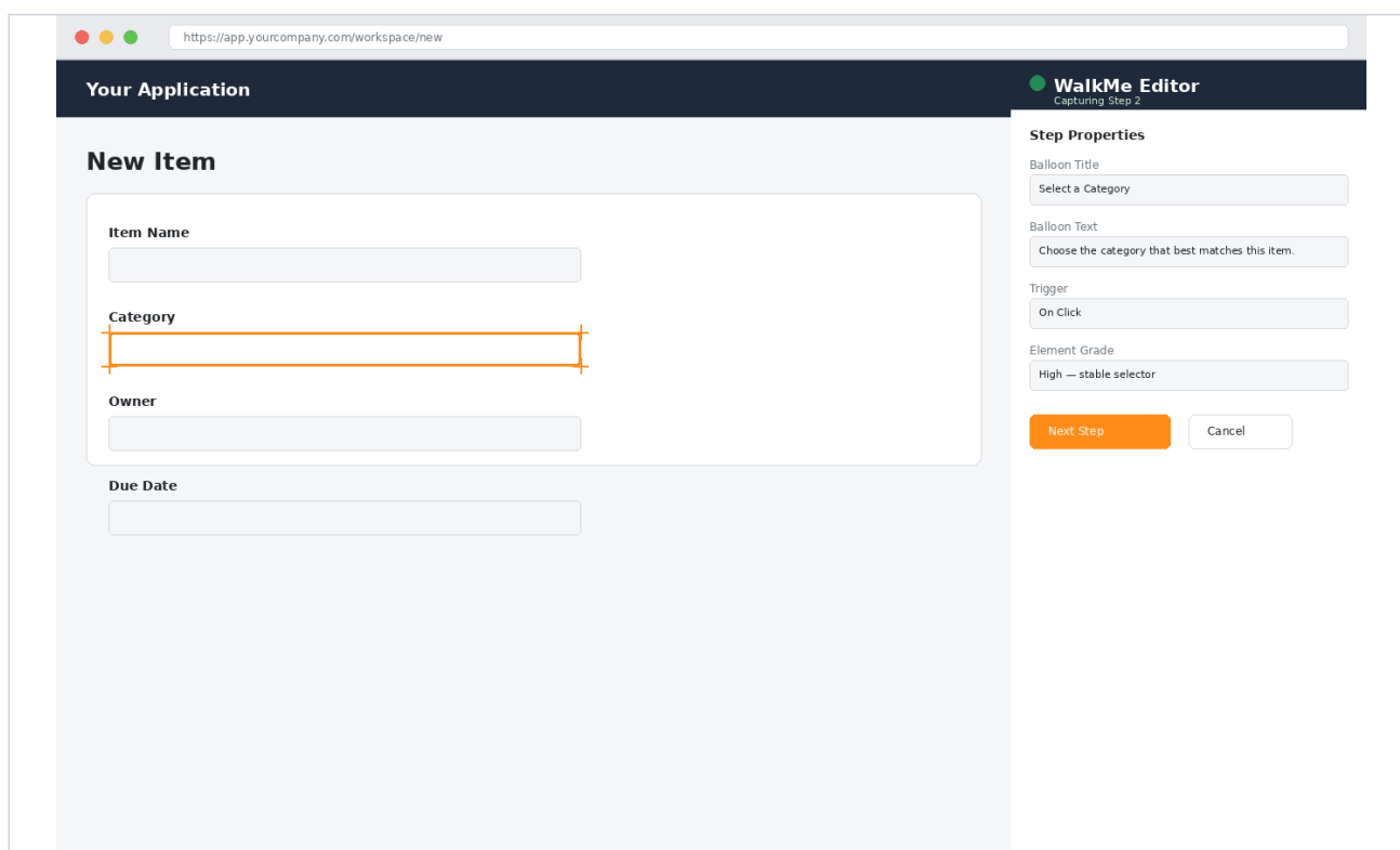
Figure 2. Capturing a step: the selected element (left) and its Step Properties panel (right).
