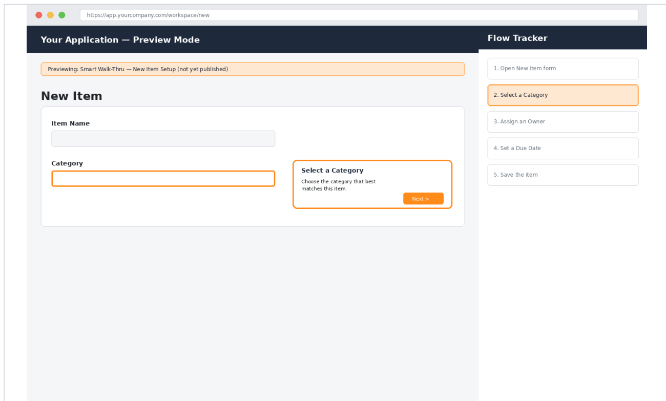
Figure 4. Preview mode with the Flow Tracker following a Smart Walk-Thru step by step.
