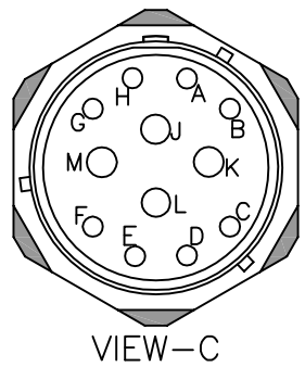
FRONT VIEW 12PIN CONTACT (MALE)
