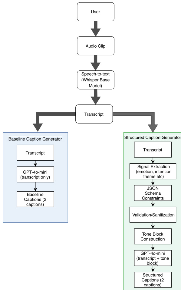
Figure 1: System architecture for transcript-only and structured signal-based caption generation
