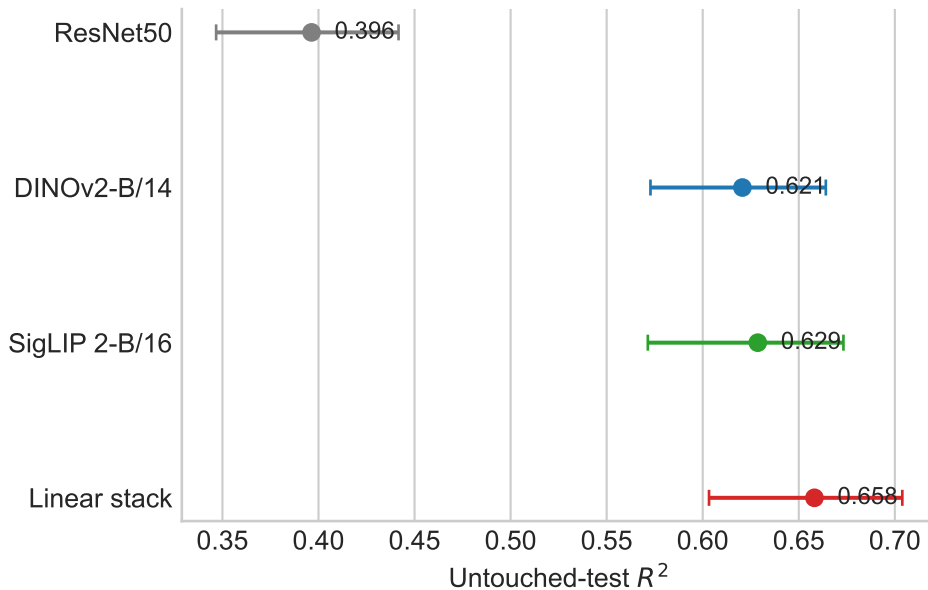
Toronto houses
