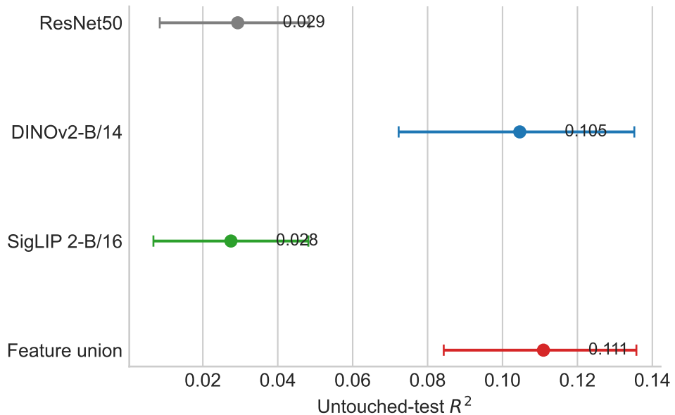
OBS horses
