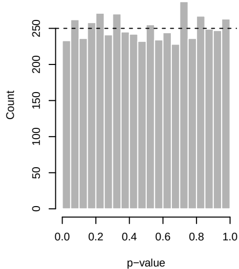
Correlated errors
