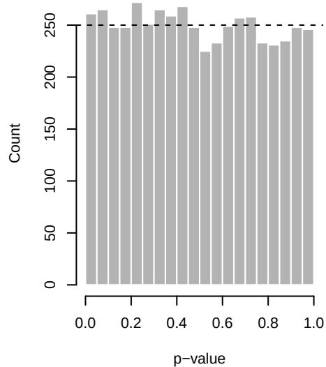
Continuous: one-per-period
