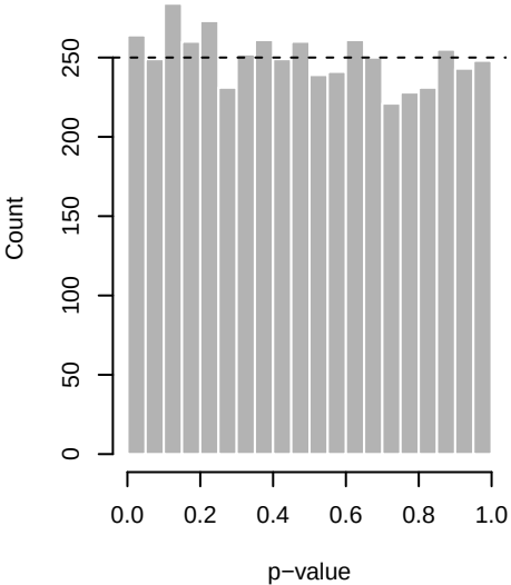
Independent errors
