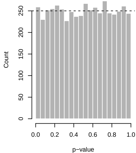
Continuous: per-sample
