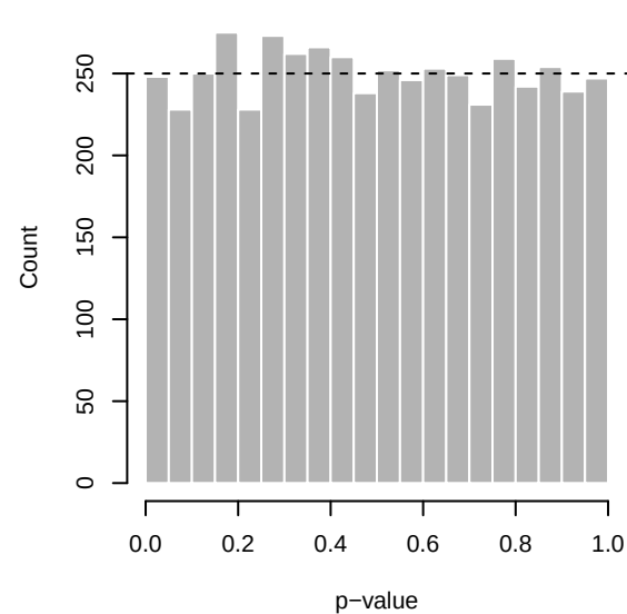
Heavy-tailed t3, HIGH count
