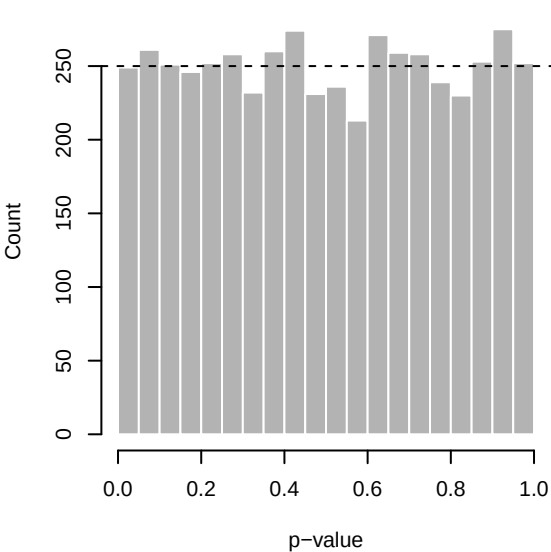
Gaussian, low count
