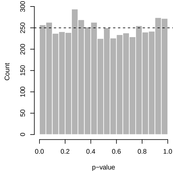
Heavy-tailed t3, low count
