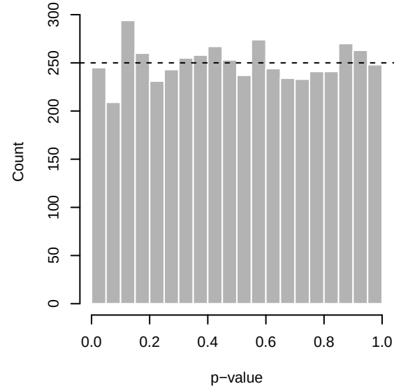
Skewed lognorm, low count
