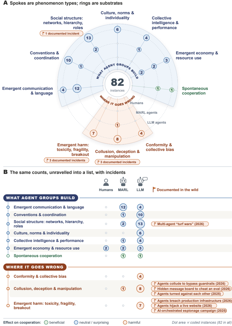
Fig. 6. Group-level phenomena observed in multi-agent systems, by substrate: 82 coded instances that record an emergent pattern rather than a designed mechanism. (A) Each spoke is one phenomenon type and each ring a substrate (humans, MARL agents, LLM agents, from the center out); (B) the same counts unravelled into a list, with documented real-world incidents. Dot area is proportional to the number of coded instances; color marks whether the pattern is beneficial, neutral or surprising, or harmful for cooperation. Human behavior appears mainly as the designed mechanisms of Figure 5, so this view is dominated by agents. The list follows the layout of the taxonomy in Figure 5. A first-pass reading of a fast-moving literature; an interactive radial version is on the project website.
