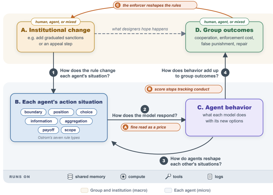
Fig. 10. A Coleman boat for agent institutions, after Coleman [21] and the question-per-arrow form of Martínez-Peña and Ylikoski [84]. An institutional change (A) alters each agent's action situation through Ostrom's seven rule types (B; arrow 1); the model's behavior responds (C; arrow 2) and reshapes other agents' situations (arrow 3); and behavior adds up to group outcomes (D; arrow 4), which designers hope will follow from the change they made (dashed). Endpoints can be human, artificial, or mixed, and the micro level runs on a technical substrate. Terracotta tags mark where the three failure modes of Fig. 9 break.
