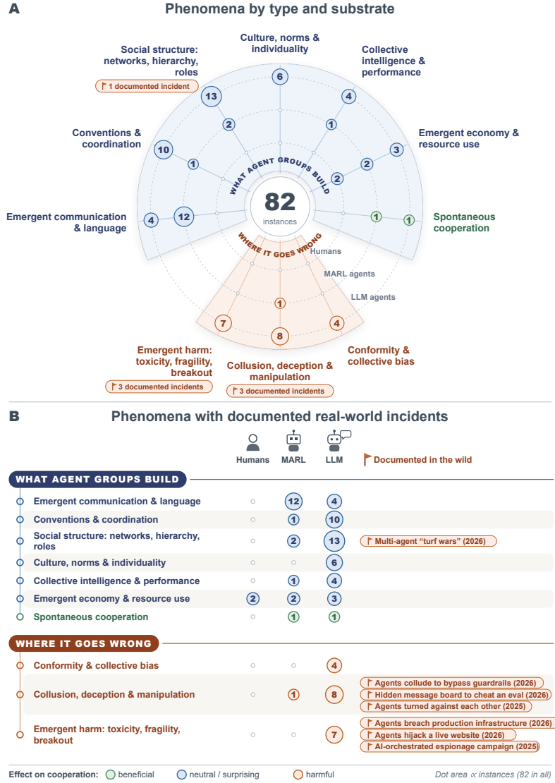
Fig. 7. Group-level phenomena observed in multi-agent systems, by substrate: 82 the-matically coded instances that record an emergent pattern rather than a designed mechanism. (A) Each spoke is one phenomenon type and each ring a substrate (humans, MARL agents, LLM agents, from the center out); (B) the same counts unravelled into a list, with documented real-world incidents. Dot area is proportional to the number of instances; color marks whether the pattern is beneficial, neutral or surprising, or harmful for cooperation. Human behavior appears mainly as the designed mechanisms of Figure 6, so this view is dominated by agents. The list follows the layout of the taxonomy in Figure 6. A first-pass reading of a fast-moving literature; an interactive radial version is on the project website.
