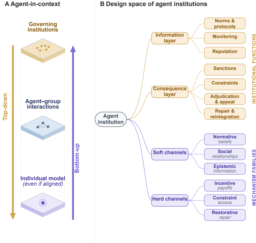
Fig. 2. Agent-in-context and the design space of agent institutions. Individual models are nested within agent-group interactions and governing institutions; institutional mechanisms shape behavior through information, consequence, and influence channels. the seven institutional functions, grouped into an information layer and a consequence layer, act on agents through six mechanism families, split into soft and hard channels.
