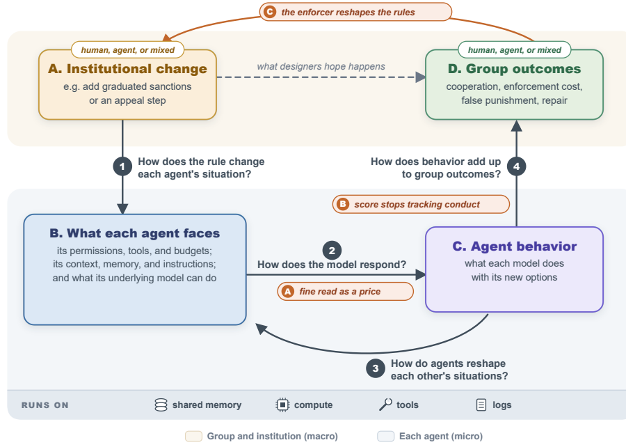
Fig. 10. A Coleman boat for agent institutions, after Coleman [16] and the question-per-arrow form of Martínez-Peña and Ylikoski [67]. An institutional change (A) alters what each agent faces (B; arrow 1); the model's behavior responds (C; arrow 2) and reshapes other agents' situations (arrow 3); and behavior adds up to group outcomes (D; arrow 4), which designers hope will follow directly from the change (dashed). Terracotta tags mark where the three failure modes of Table 3 break.
