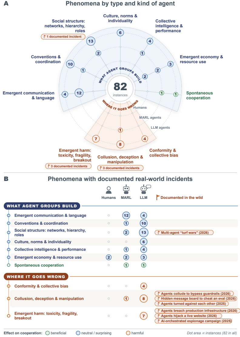
Fig. 7. Group-level phenomena in multi-agent systems, by kind of agent: 82 coded instances that record an emergent pattern rather than a designed mechanism. (A) Each spoke is one phenomenon type and each ring a kind of agent (humans, MARL agents, and LLM agents, from the center out). (B) The same counts as a list, with documented real-world incidents. Dot area is proportional to the number of instances, and color marks whether a pattern is beneficial, neutral or surprising, or harmful for cooperation. Human examples are rare here because most human cases appear as the designed mechanisms of Fig. 6.
