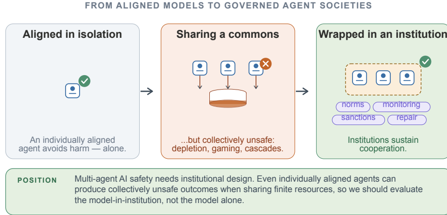
Fig. 1. [Figure to be redesigned before press.] The paper’s position in one view. Left: an individually aligned agent avoids harm on its own. Center: the same agents sharing a finite commons can still fail collectively—through resource depletion, reputation gaming, and cascading errors. Right: institutional mechanisms (norms, monitoring, sanctions, repair) wrapped around the agents sustain cooperation. We argue that multi-agent AI safety should evaluate the model-in-institution , not the model alone.
