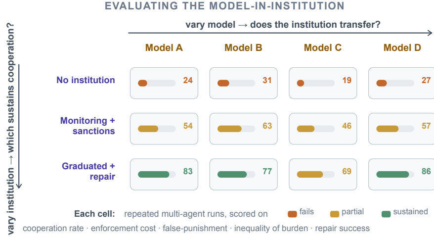
Fig. 6. [Figure to be redesigned before press.] The model-in-institution evaluation design. Each cell aggregates repeated multi-agent runs of one model under one institution, scored on the metrics of Table 1 (colour indicates whether cooperation is sustained). Reading across a row holds the institution fixed and varies the model (does the mechanism transfer?); reading down a column holds the model fixed and varies the institution (which institution sustains cooperation?). Cell scores are illustrative.
