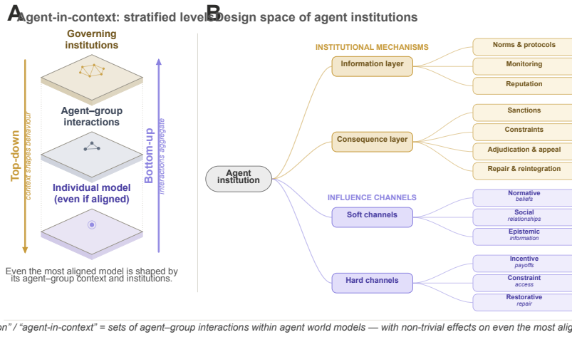
Fig. 3. Agent-in-context and the design space of agent institutions. Individual models are nested within agent-group interactions and governing institutions; institutional mechanisms shape behavior through information, consequence, and influence channels.
