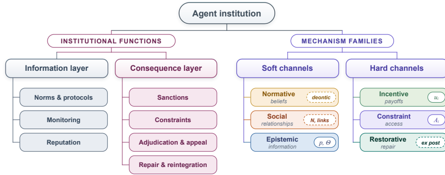
Fig. 5. The design space of agent institutions. Institutional functions (left) say what an institution must do, in an information layer (grey) and a consequence layer (plum). Mechanism families (right) say how it acts on agents, through soft and hard channels, in the colors of Fig. 6. Badges mark the part of a Bayesian game \mathcal{G} = (N, A_i, \Theta_i, p, u_i) that each family changes (solid), or what it adds beyond the one-shot game (dashed).
