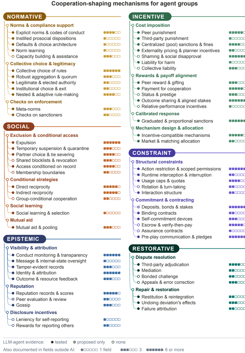
Fig. 6. Cooperation-shaping mechanisms for agent groups: 66 mechanisms in 18 themes, thematically coded from 645 instances across AI and 18 other disciplines (Section 3) and grouped by the six mechanism families. Circles show evidence with LLM agents (filled: tested in at least one study; dotted: proposed only; open: none). Squares count the fields outside AI in which a mechanism is also documented; six filled squares means six or more.
